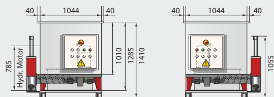
Left version
