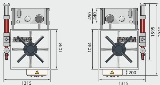
Right version
